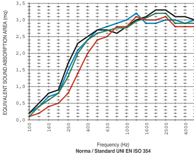
ONE-THIRD-OCTAVE EQUIVALENT SOUND ABSORPTION AREA Aobj CURVE
